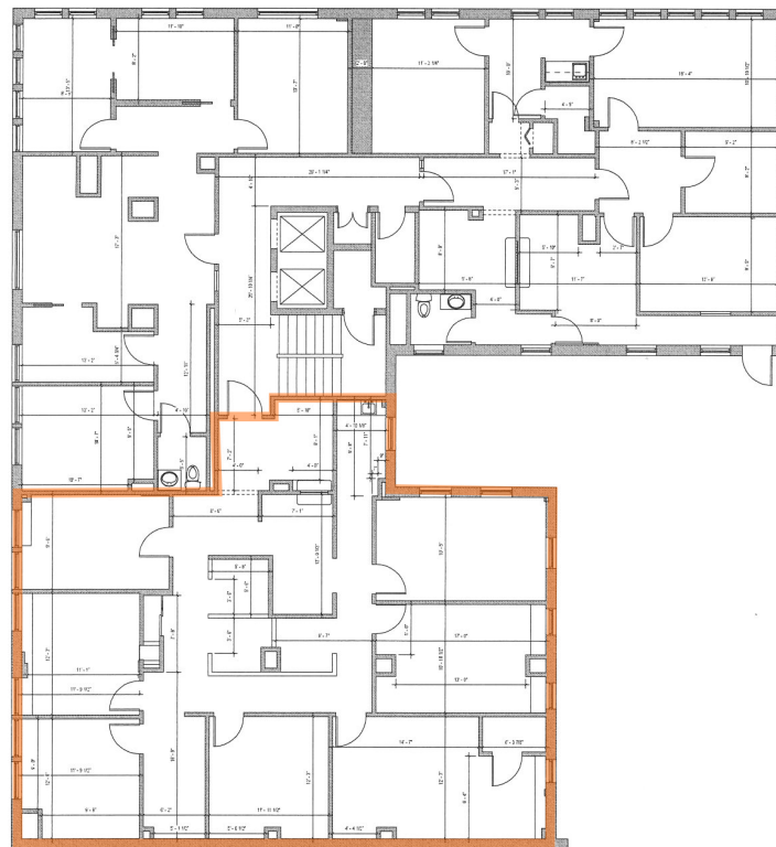
Courtside Building - 2nd Floor Plan 11-1-12
